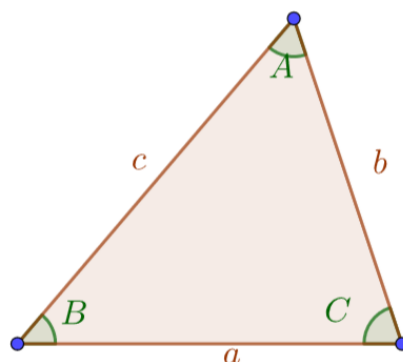
Figura 3.7: Triangle no rectangle
